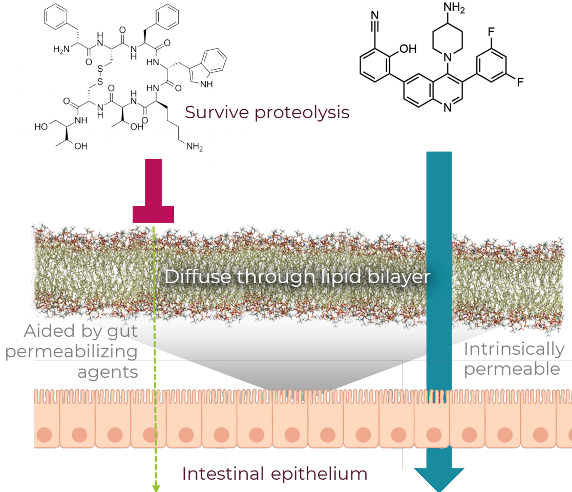
Nonpeptide: paltusotine
